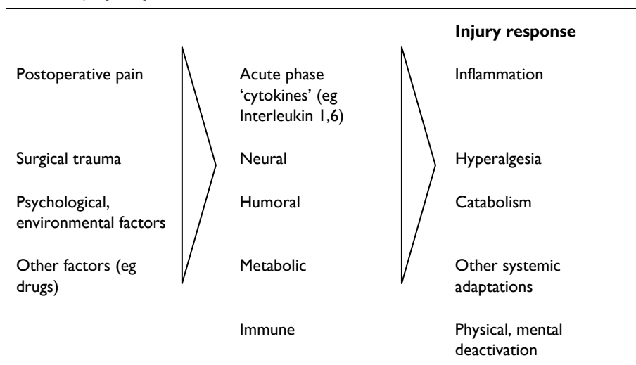
Figure 1.2 The injury response
